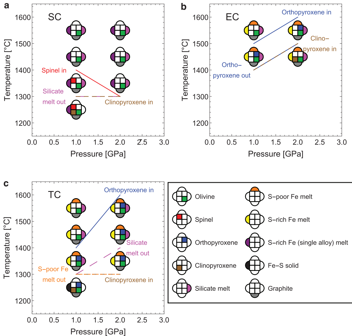
FIG. 2. Phase diagrams of SC (a), EC (b), and TC (c) run products. Solid and dashed lines represent major phase changes in the direction of lower temperatures. SC = sequential condensation chemistry, EC = equilibrium chemistry, TC = third bulk composition based on equilibrium chemistry.
